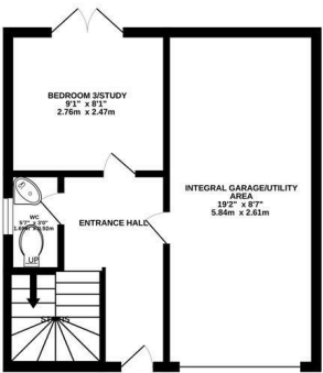
GROUND FLOOR 338 sq.ft. (31.4 sq.m.) approx.
