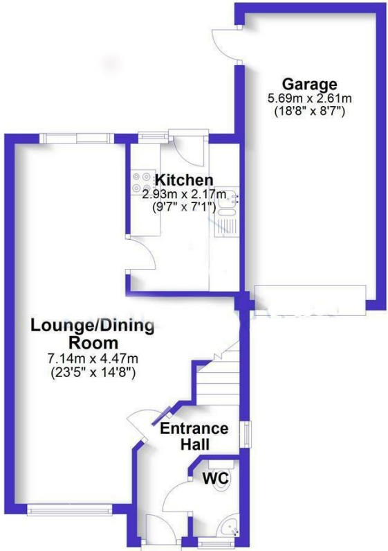
Ground Floor Approx. 48.2 sq. metres (518.6 sq. feet)
