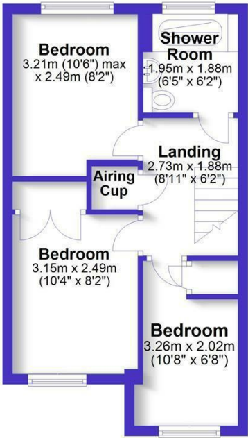
First Floor Approx. 33.8 sq. metres (363.3 sq. feet)
