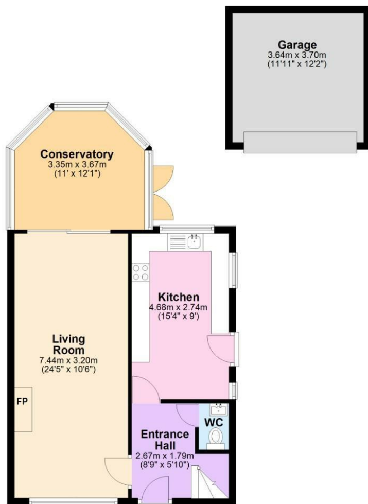
Ground Floor Approx. 69.9 sq. metres (752.0 sq. feet)
