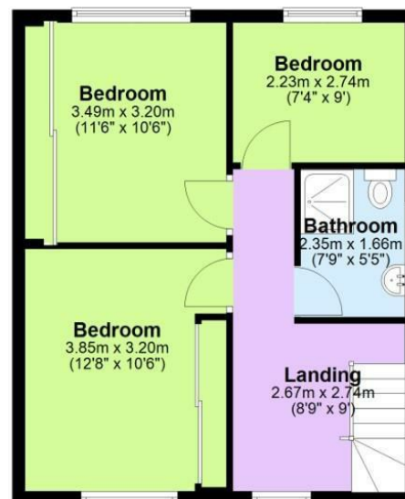
First Floor Approx. 45.0 sq. metres (484.2 sq. feet)
