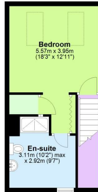
Second Floor Approx. 31.3 sq. metres (337.0 sq. feet)
