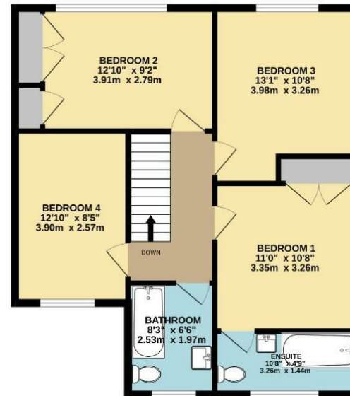
1ST FLOOR 678 sq.ft. (63.0 sq.m.) approx.
