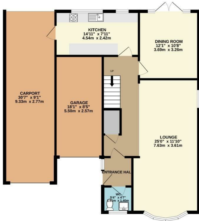
GROUND FLOOR 1118 sq.ft. (103.9 sq.m.) approx.
