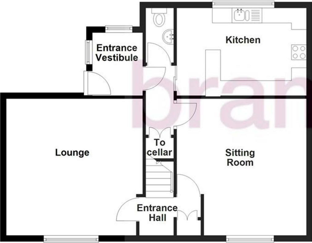
Ground Floor
