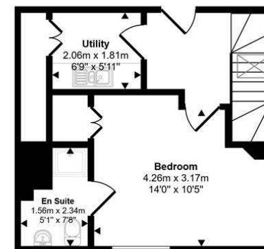
First Floor Approx 32 sq m / 346 sq ft
