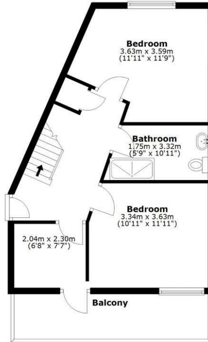
Ground Floor Approx. 47.5 sq. metres (511.5 sq. feet) (excluding Balcony)
