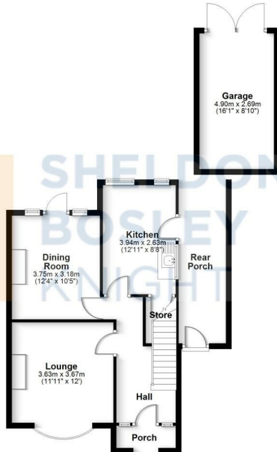
Ground Floor Approx. 73.0 sq. metres (785.3 sq. feet)
