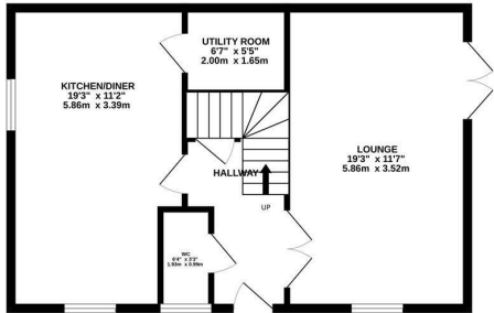
GROUND FLOOR 562 sq.ft. (52.3 sq.m.) approx.
