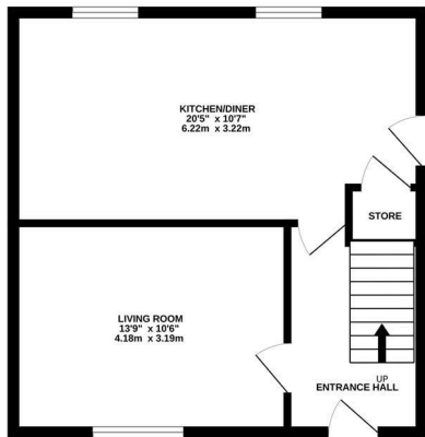
GROUND FLOOR 429 sq.ft. (39.9 sq.m.) approx.
