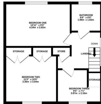
1ST FLOOR 429 sq.ft. (39.9 sq.m.) approx.
