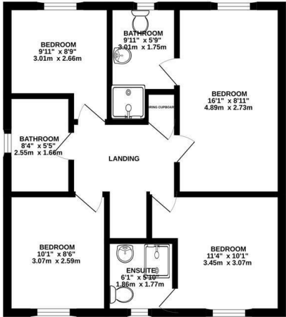
1ST FLOOR 612 sq.ft. (56.8 sq.m.) approx.
