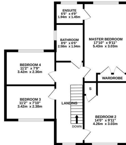
1ST FLOOR 693 sq.ft. (64.4 sq.m.) approx.
