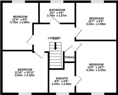
1ST FLOOR 678 sq.ft. (63.0 sq.m.) approx.
