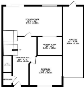
GROUND FLOOR 612 sq ft. (56.9 sq.m.) approx.
