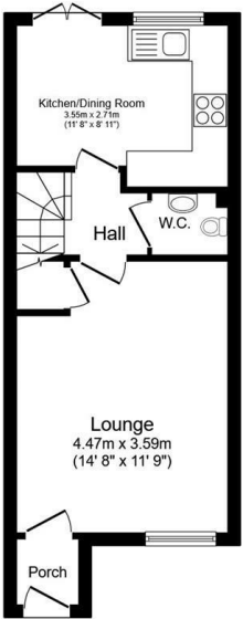
Ground Floor
