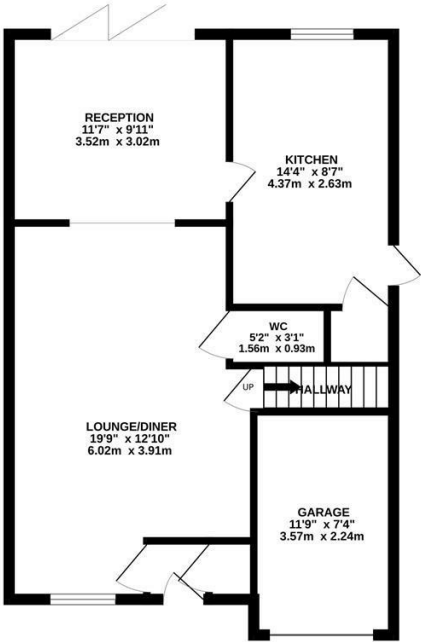
GROUND FLOOR 612 sq.ft. (56.9 sq.m.) approx.
