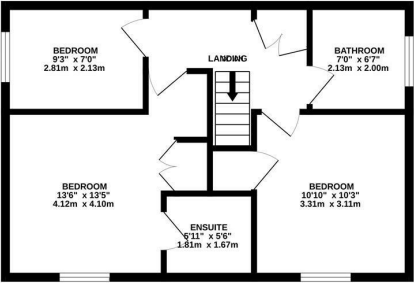
1ST FLOOR 474 sq.ft. (44.0 sq.m.) approx.
