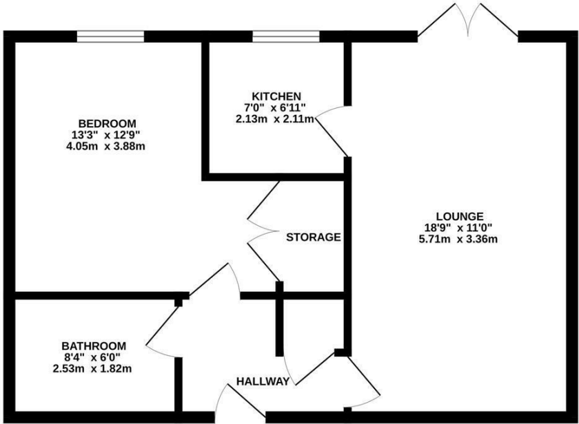
GROUND FLOOR 518 sq.ft. (48.1 sq.m.) approx.
