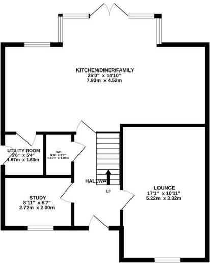
GROUND FLOOR 695 sq.ft. (64.6 sq.m.) approx.
