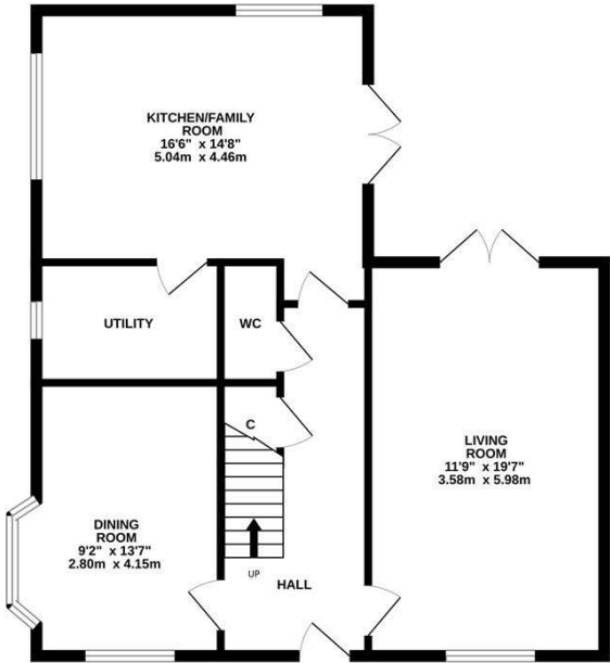
GROUND FLOOR 768 sq.ft. (71.4 sq.m.) approx.
