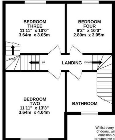
TOTAL FLOOR AREA : 1645 sq.ft. (152.8 sq.m.) approx.
