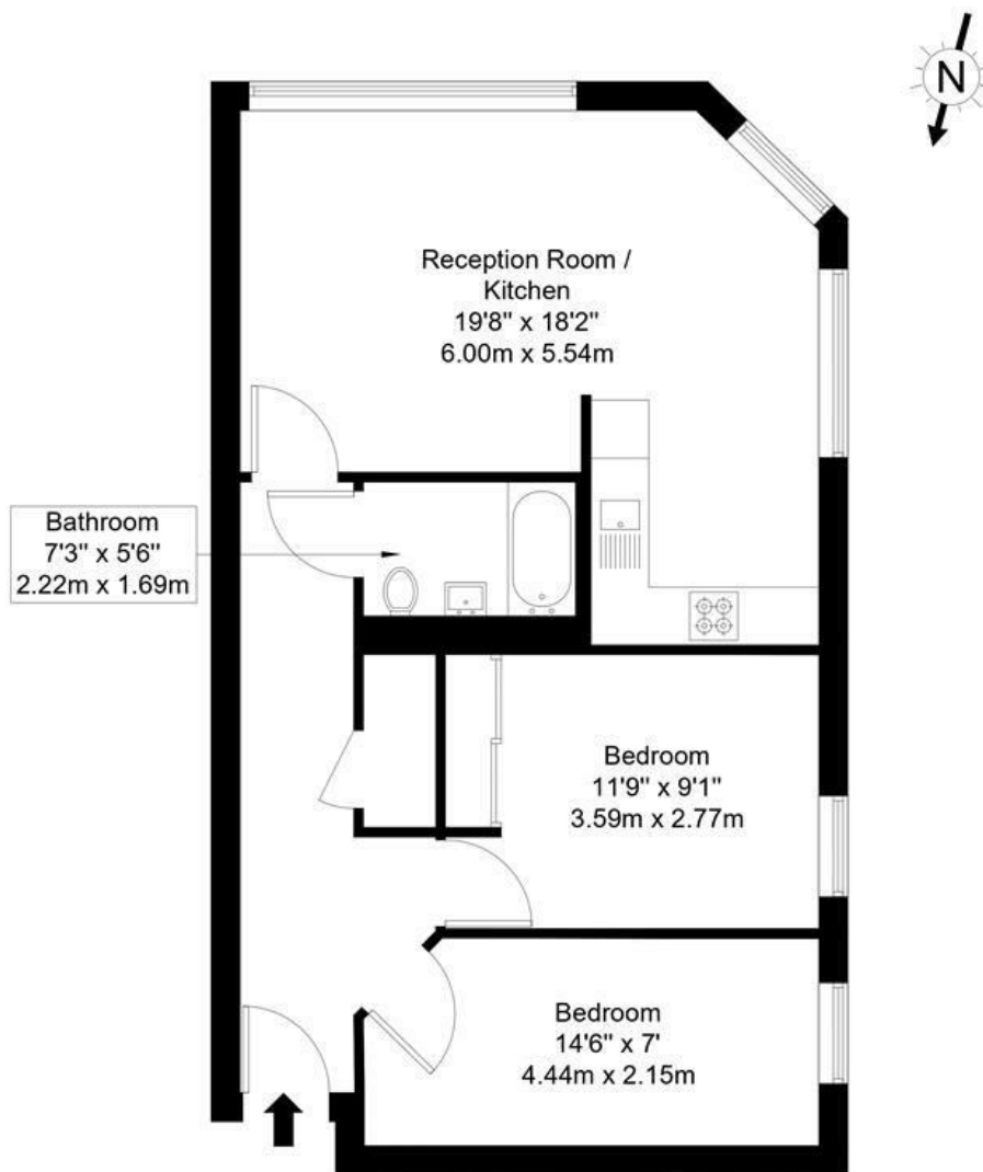
First Floor
