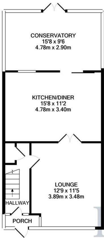
GROUND FLOOR APPROX. FLOOR AREA 536 SQ.FT. (49.8 SQ.M.)
