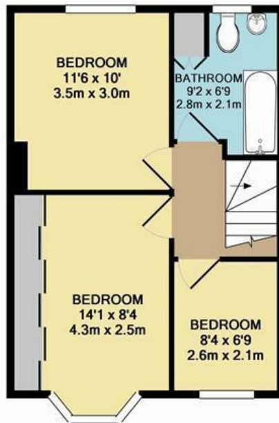
1ST FLOOR APPROX. FLOOR AREA 402 SQ.FT. (37.4 SQ.M.)
