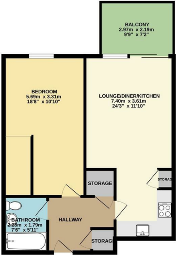
TOTAL FLOOR AREA: 55.8 sq.m. (603 sq.ft.) approx. Whilst every attempt has been made to ensure the accuracy of the floorplans contained herein, measurements of plots, sections, corners and any other items are approximate and are not intended to be taken as any form of guarantee or warranty. The floorplans are for illustrative purposes only and should be used as a guide only. The prospective purchaser should verify the accuracy of the floorplans and should be satisfied with the plan before purchase. The floorplans, sections and any other items shown have not been tested and the purchaser should verify the accuracy of the floorplans and should be satisfied with the plan before purchase. Made with SketchUp 2018
