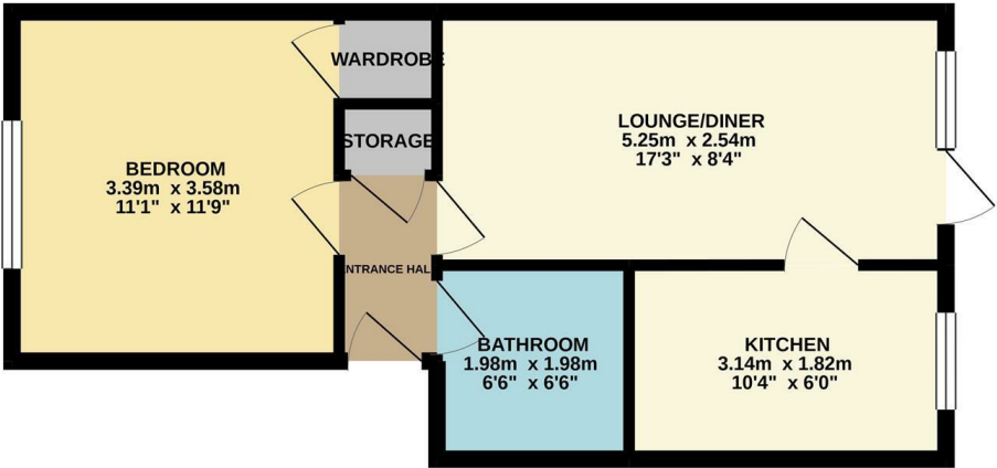
GROUND FLOOR 40.1 sq.m. (431 sq.ft.) approx.
