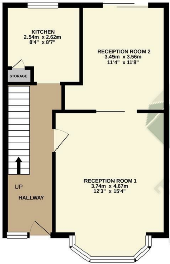
GROUND FLOOR 43.0 sq.m. (462 sq.ft.) approx.
