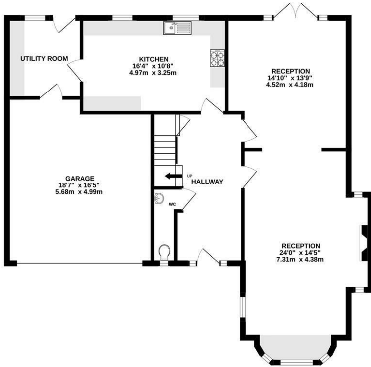
GROUND FLOOR 1216 sq.ft. (113.0 sq.m.) approx.
