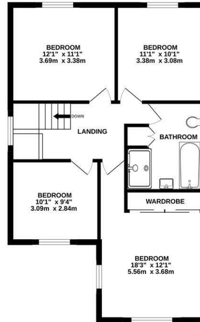
1ST FLOOR 720 sq.ft. (66.9 sq.m.) approx.
