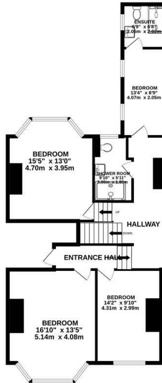
GROUND FLOOR 886 sq.ft. (82.3 sq.m.) approx.
