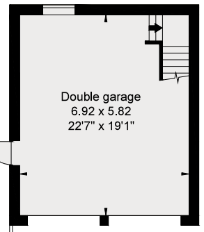
Outbuilding Ground Floor Shown in actual location / orientation
