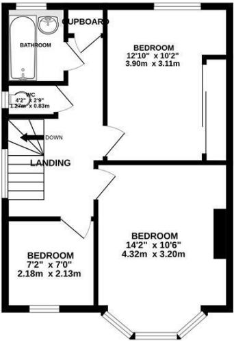
1ST FLOOR 466 sq.ft. (43.3 sq.m.) approx.
