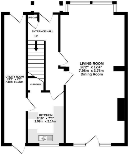
GROUND FLOOR 573 sq.ft. (53.3 sq.m.) approx.
