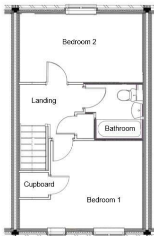
First Floor Bedroom 1 4.62m x 3.32m Bedroom 2 4.62m x 2.60m Bathroom 2.16m x 2.03m
