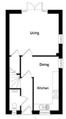
Ground Floor KITCHEN / DINING 4.50m x 3.50m 14'9" x 11'6"
