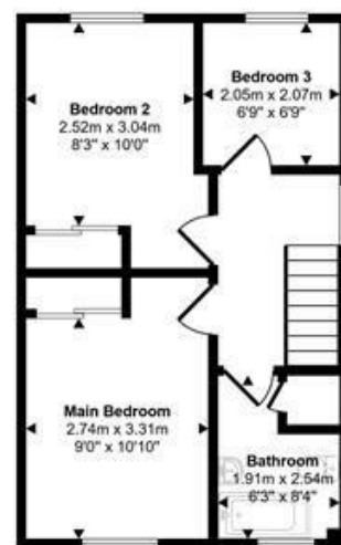
First Floor Approx 37 sq m / 397 sq ft
