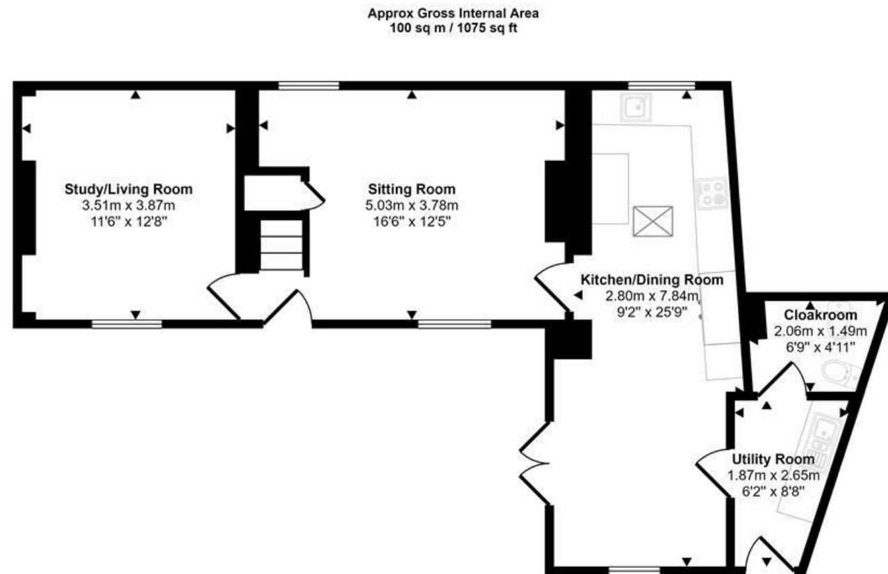
Ground Floor Approx 64 sq m / 693 sq ft
