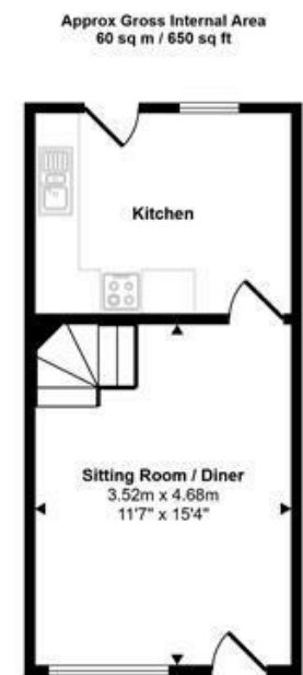
Ground Floor Approx 27 sq m / 289 sq ft
