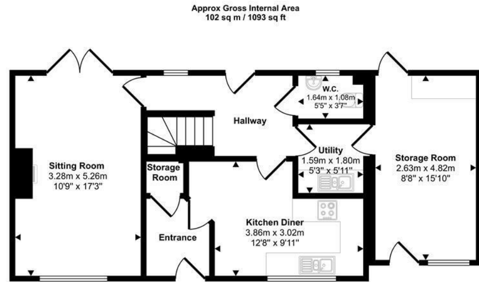
Ground Floor Approx 62 sq m / 663 sq ft
