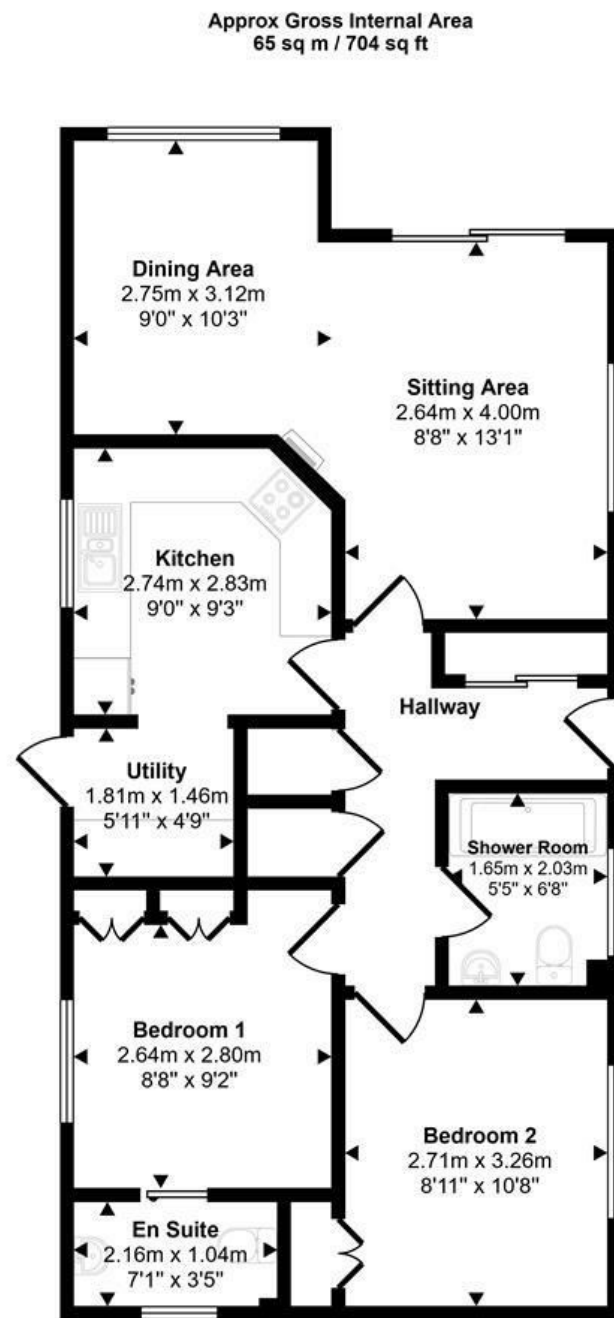
Floorplan
