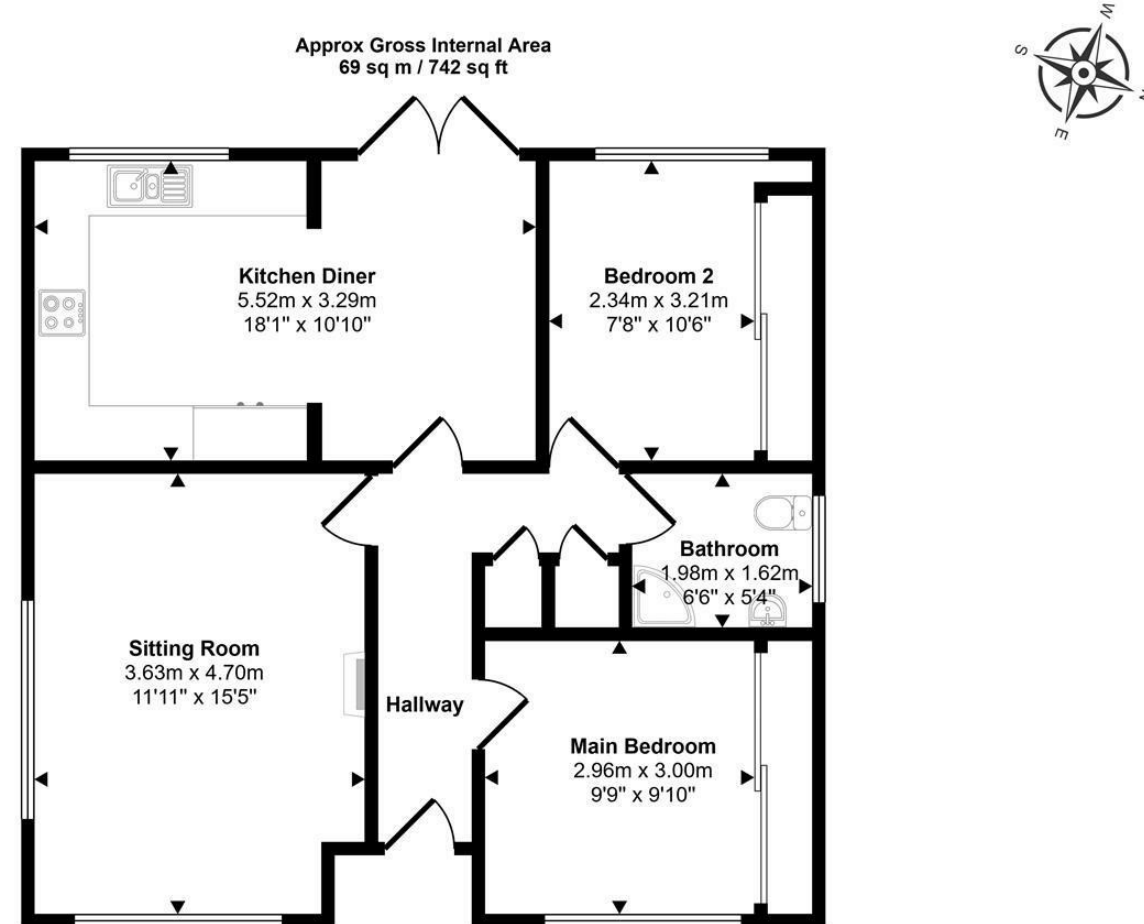
Floorplan
