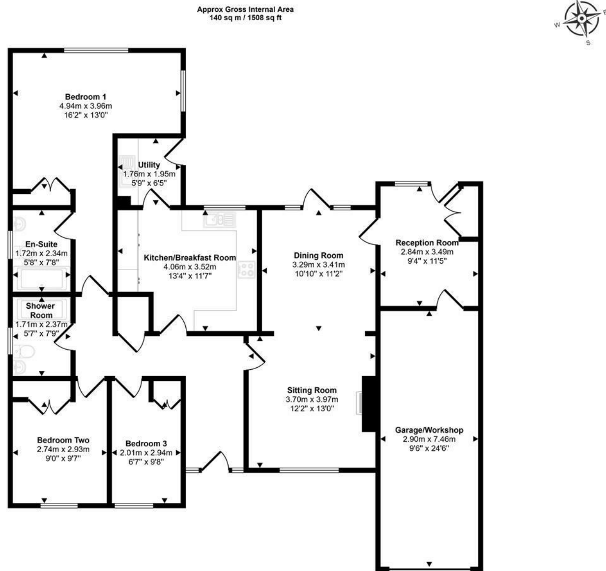
Floorplan
