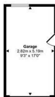
Garage Approx 15 sq m / 157 sq ft
