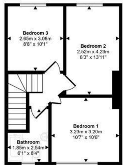
First Floor Approx 40 sq m / 431 sq ft
