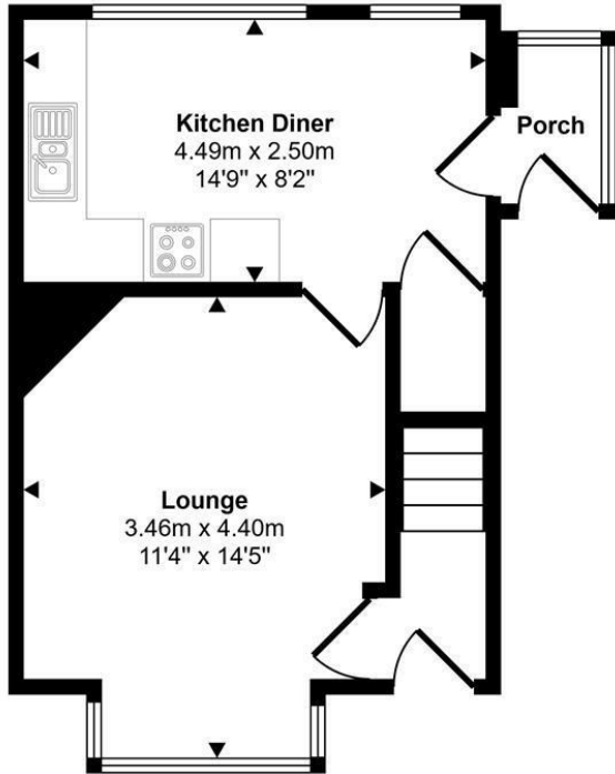
Ground Floor Approx 31 sq m / 336 sq ft
