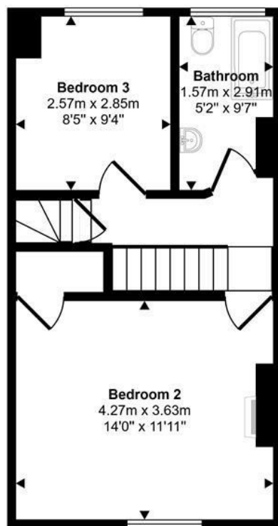
First Floor Approx 36 sq m / 384 sq ft
