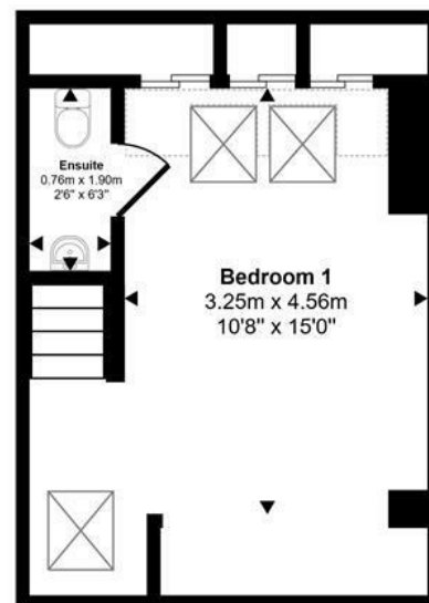
Second Floor Approx 26 sq m / 280 sq ft
