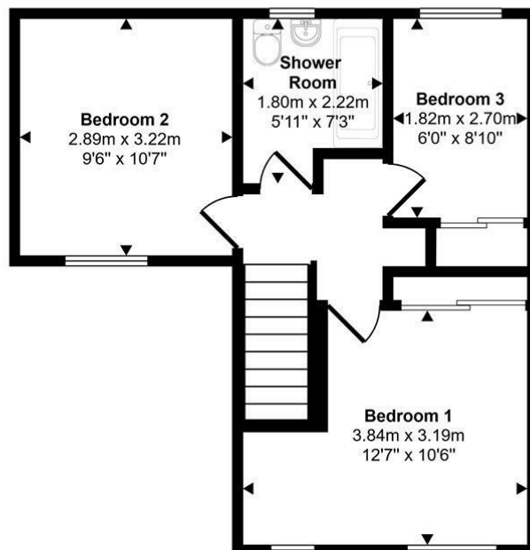
First Floor Approx 37 sq m / 401 sq ft
