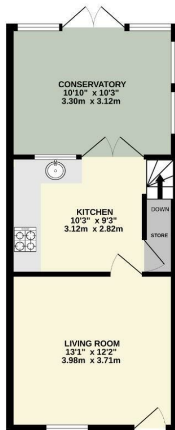
GROUND FLOOR 414 sq.ft. (38.5 sq.m.) approx.
