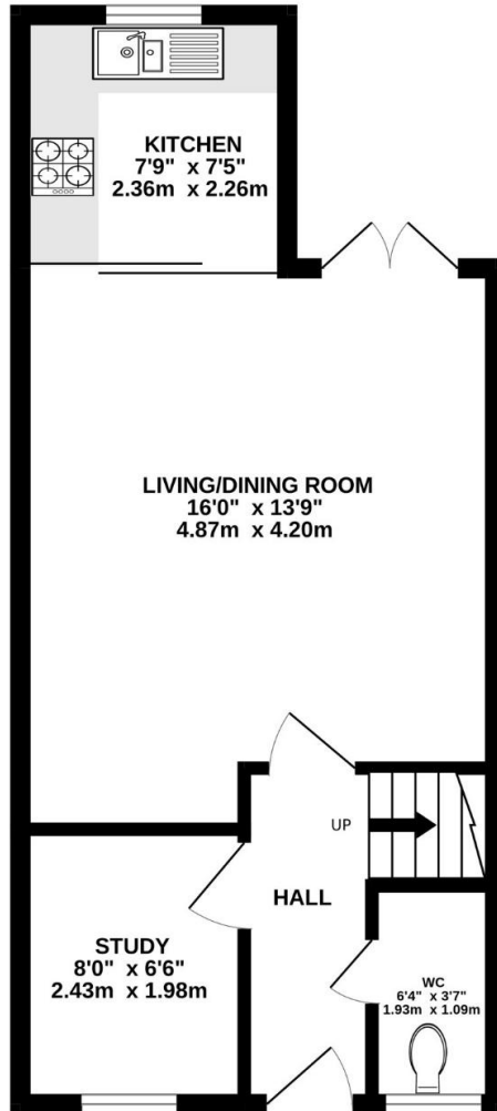
GROUND FLOOR 391 sq.ft. (36.3 sq.m.) approx.
