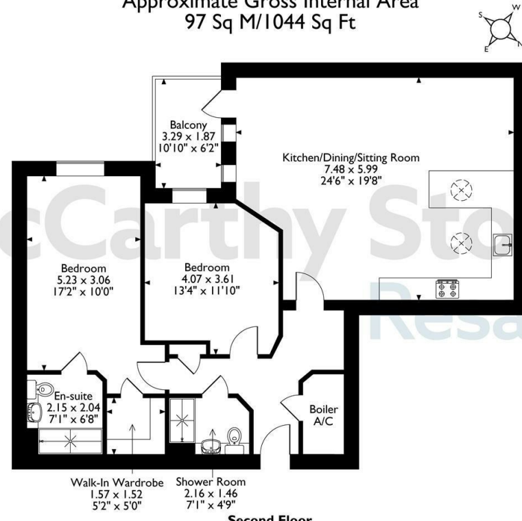
Second Floor The position & size of doors, windows, appliances and other features are approximate only. © ehouse. Unauthorised reproduction prohibited. Drawing ref. dig/8662191/DST.
